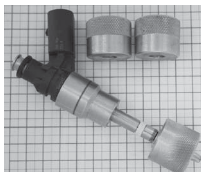
INJECTOR LOWER SEAL COMPRES- SION FITTING SET
