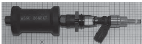
Adjustable Puller & Slide Hammer
