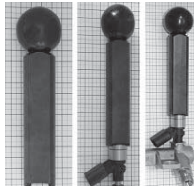
FUEL RAIL INJECTOR REFITTING TOOL
